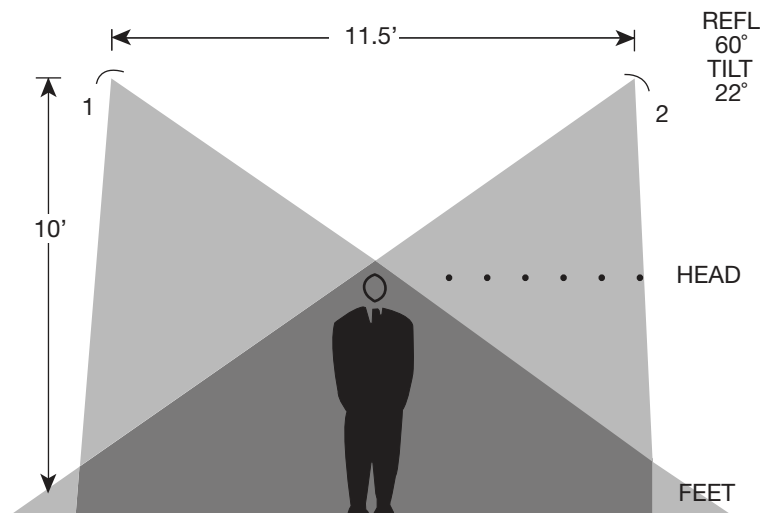
Figure 4: Typical Infrared Heating Pattern
