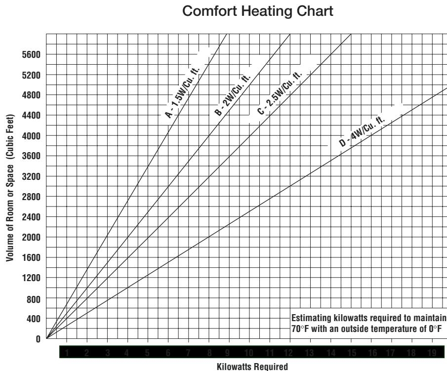
Graph 1: Quick Estimation Chart for Various Room Heat Loss Conditions
