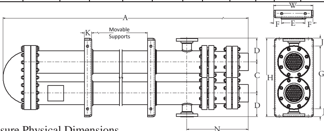
Separated Closure Physical Dimensions
