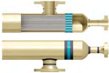
Fixed tubesheet design, non-removable channel.
