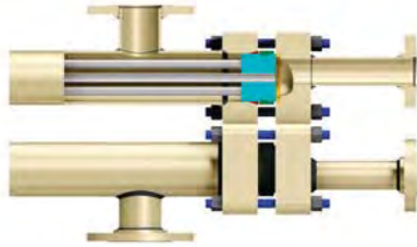
Holland standard closure. Tube nozzles can be offset for venting and draining. ANSI flange connections.
